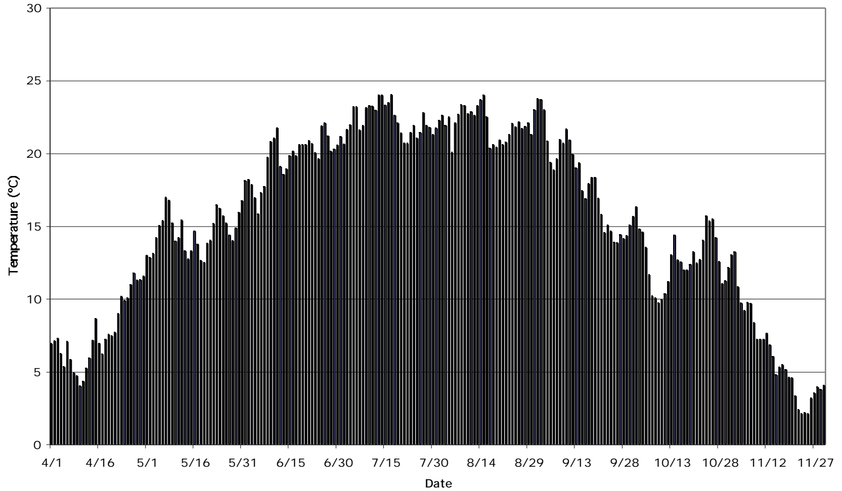
Fig. 3. Average Daily Soil Temperature, O.J. Noer Turfgrass Research Facility, Verona, WI, 2000.
